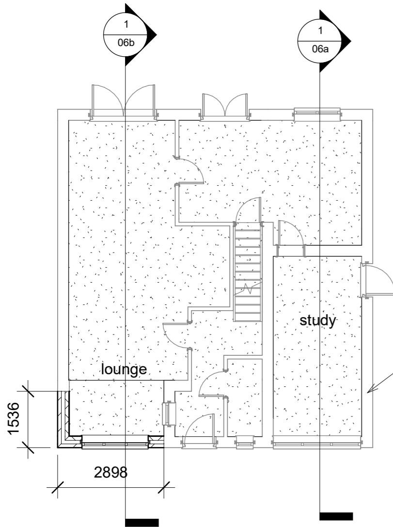
1 Proposed ground floor plan 1 : 100
